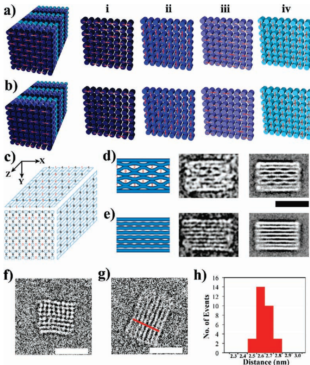
Figure 3. Cryo-EM images of the 8 \times 8 square lattice. (a) Three-dimensional cylinder model of a hypothetical 8 \times 8 square lattice with all default staple crossovers intact. Cross-sectional slices i to iv (parallel to the xy -plane, spaced at 8-bp intervals) reveal that each slice retains 28 crossovers (short line in red), evenly distributed across the xy -plane. The crossovers in i and iii sectional slices are parallel to the xz -plane, while the crossovers in ii and iv sectional slices are parallel to the yz -plane. (b) 3D cylinder model of an 8 \times 8 square lattice in which crossovers have been systematically omitted from i and iii sectional slices. This design decreases the density of crossovers parallel to the xz -plane. (c) Diagram illustrating the distribution of crossovers in the 8 \times 8 square lattice along xy -, xz -, and yz -projections. As a result of the omissions of crossovers parallel to the xz -plane, the numbers of crossovers along lines parallel to the y -axis are significantly smaller at certain positions (number of crossovers indicated in red). (d) Left to right: predicted model of 8 \times 8 square lattice in xz -projection; cryo-EM image of a single particle; and averaged image of 45 particles showing the side view corresponding to the xz -projection. (e) Left to right: predicted model of 8 \times 8 square lattice in yz -projection; cryo-EM image of a single particle; and averaged image of 70 particles showing the side view corresponding to the yz -projection. (f) Cryo-EM image of a particle showing the end view corresponding to the xy -projection. (g) Cross-section analysis of the images gives the width of the construct from which the periodicity of the helices in the structure can be obtained. (h) Narrow distribution of helical widths centered at 2.6 nm. Scale bars in d-g: 20 nm.
